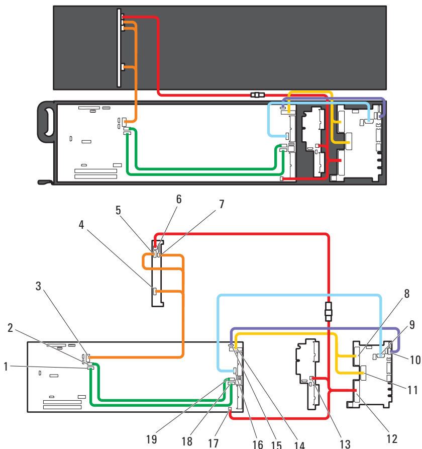
图 3-31. 热插拔硬盘驱动器背板的电缆布线情况
